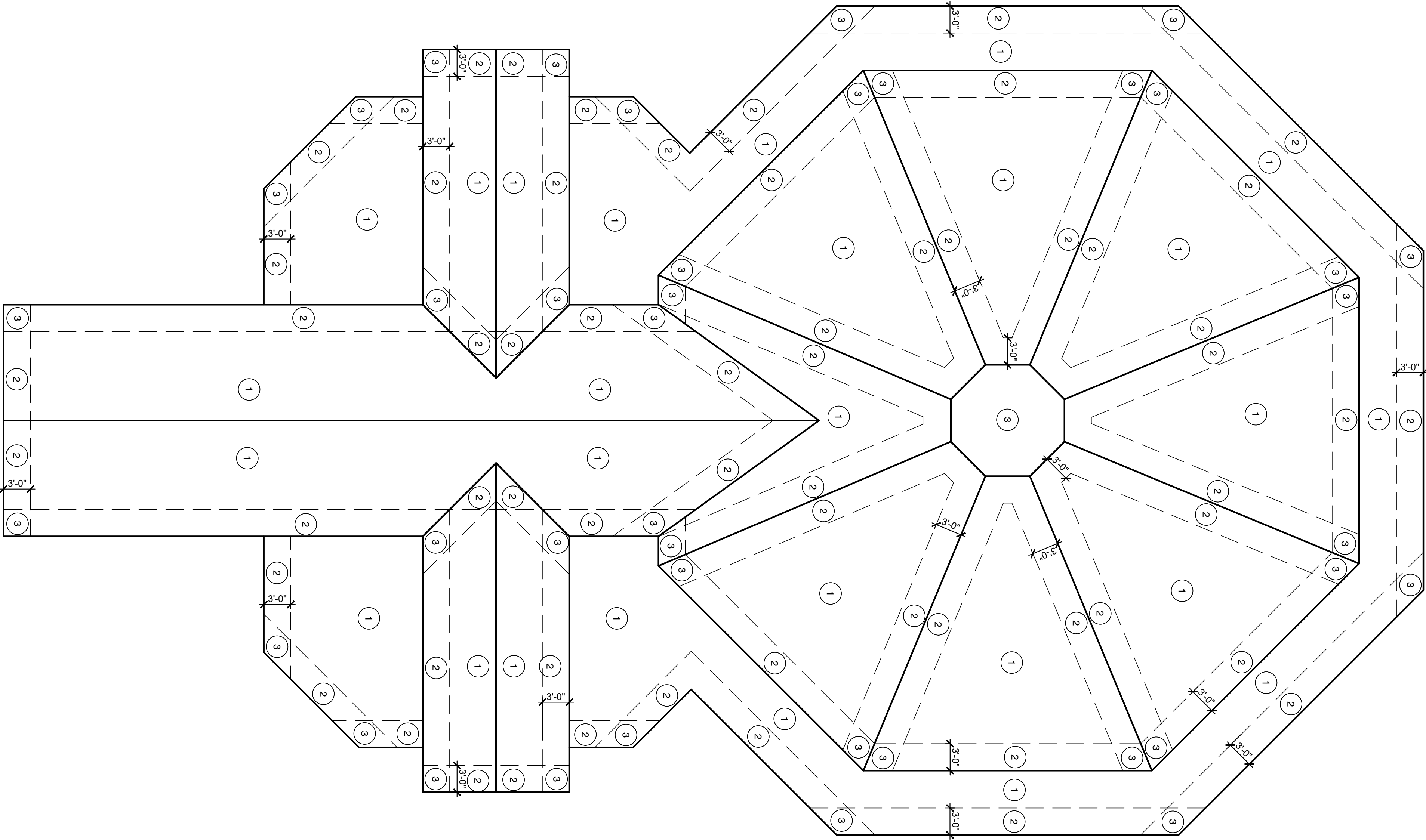
PROPOSED ROOF ZONE PLAN SCALE: 1/8" = 1'-0" (PRINTED @ 24X36) SCALE: NTS = (PRINTED @ 11X17)
