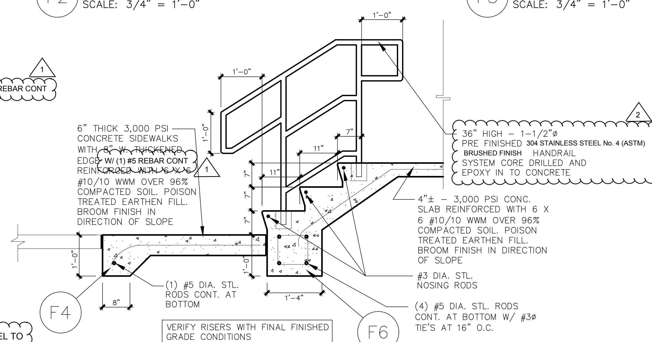
F2 SECTION CUT AT STAIRS SCALE: 3/4" = 1'-0"
