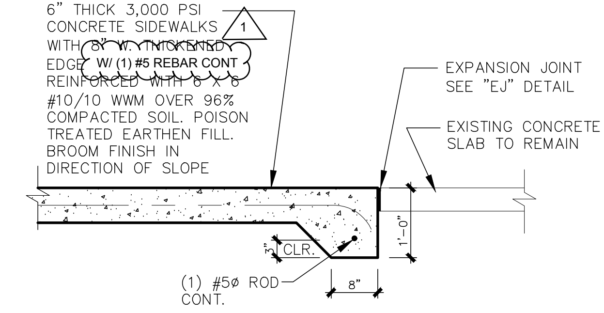
F4 THICKENED EDGE TO EXISTING CONCRETE SIDEWALK SCALE: 3/4" = 1'-0"
